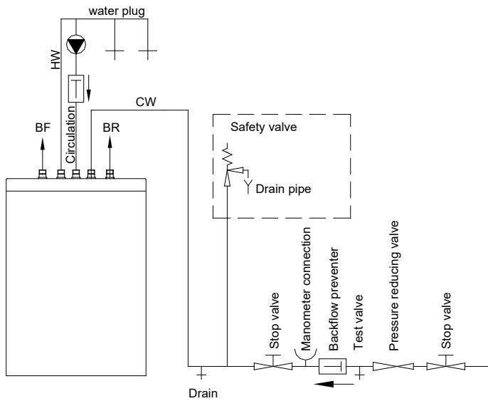
Connection Scheme (according to DIN 1988)
